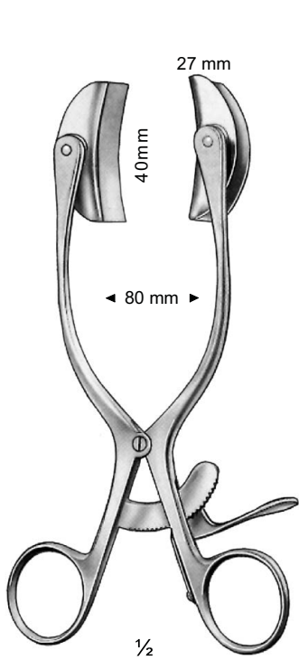
Baby-Collin 401-01 17 cm / 6¾" Abdominal retractor complete with 2 pairs of blades
