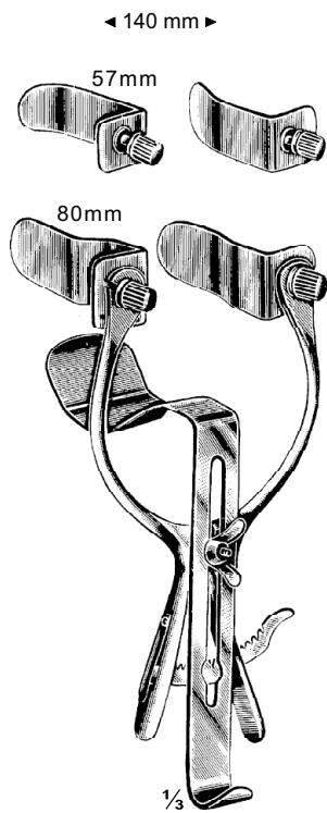
Millin 416-01 19.5 cm / 7¾" 2 pairs of lateral blades and 1 central blade
