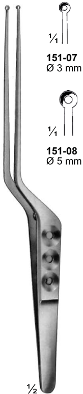
Yasargil 151-07 & 151-08 20 cm / 8" Spoon type sharp
